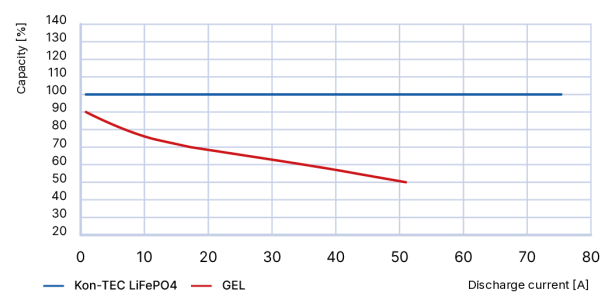
Fig. 5. Capacity comparison of Kon-TEC LiFePO 4 and lead-acid batteries at different discharge currents
