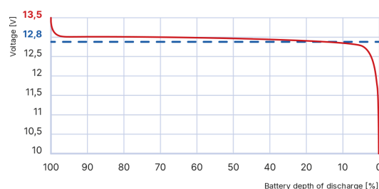
Fig. 1. Battery voltage drop, 1C discharge
