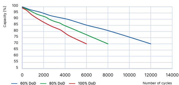
Fig. 3. Battery cycle life at different depths of discharge (DoD). 1C discharge current
