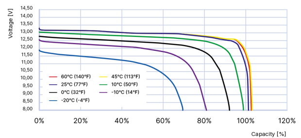
Fig. 4. Battery voltage during discharge at different temperatures. 1C discharge current
