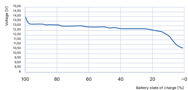
Fig. 7. Battery voltage during discharge at different states of charge (SoC). 0.1C discharge current
