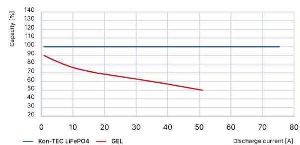
Fig. 5. Capacity comparison of Kon-TEC LiFePO 4 and lead-acid batteries at different discharge currents
