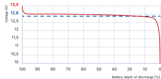
Fig. 1. Battery voltage drop, 1C discharge
